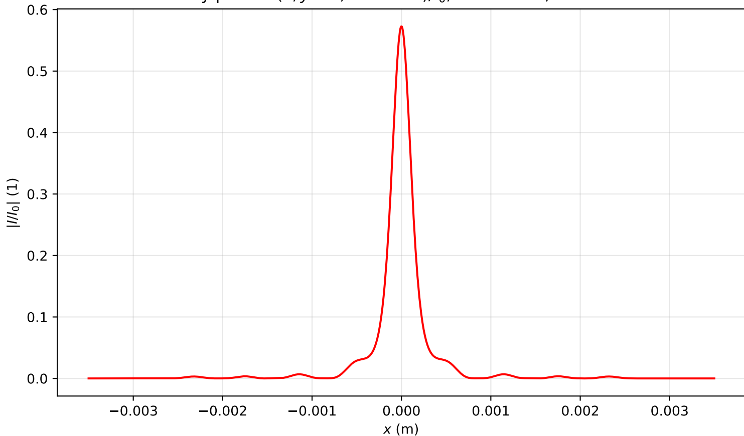
Intensity profile I(x, y = 0, z = 3.981)/I_0 , P_{in}=7.0P_{cr} , artificial time
